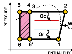
Fig. 2 EXTRA FREE CAPACITY WITH SUBCOOLER
