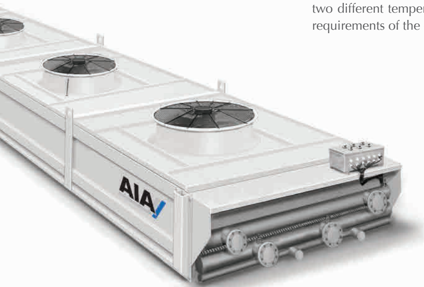
Configuration with two circuits (LT, HT)
